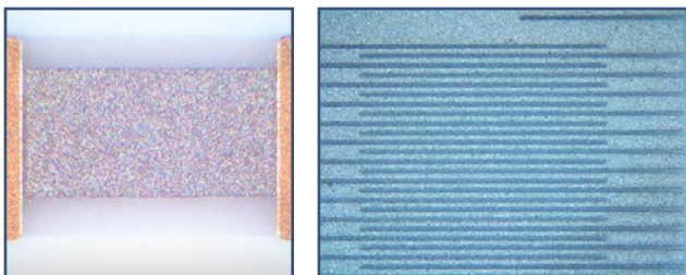
Symmetric shave trim (L) and dense serpentine pattern (R) in thin film on alumina with the green laser.
